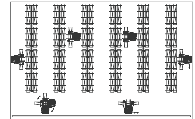
Long material storage mode Multi direction forklift
